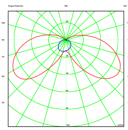
airy evolution 1x26W
