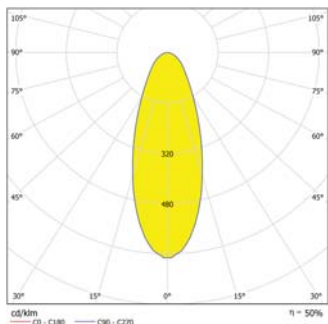
1X70W CDM-T WIDE BEAM
