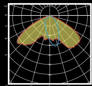
ARRO VIA 250W HPS (CLEAR)
