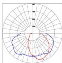
Maximum Candela = 571, Location At Horizontal Angle = 0°, Vertical Angle = 87.5° Minimum Beam Candela Maximum Candela = 579, Location At Horizontal Angle = 90°, Vertical Angle = 87.5° Minimum Beam Candela Maximum Candela = 579, Location At Horizontal Angle = 90°, Vertical Angle = 87.5° Minimum Beam Candela
