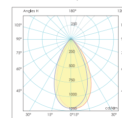
Photometry ~ 300W
